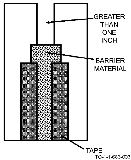
Figure 4-2. Tape and Barrier Material Application
