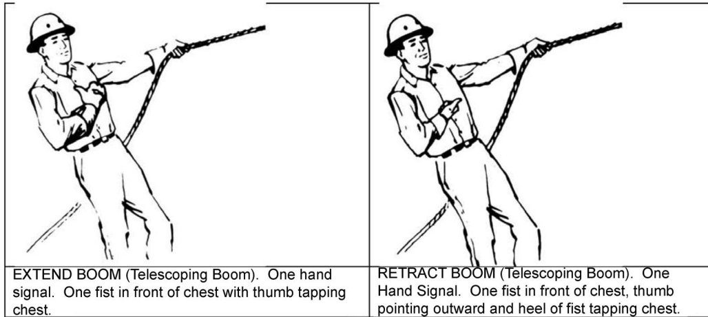
Figure 10-1. Hand Signals for Crane Operation (Sheet 3)
