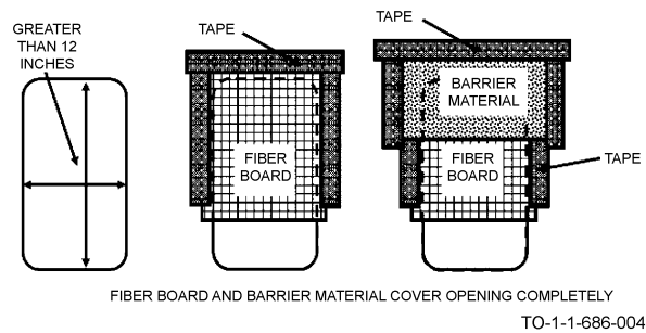
Figure 4-3. Sealing Openings Greater Than 12 Inches
