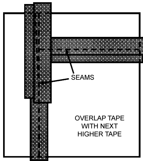
Figure 4-5. Overlapping Tape Application
