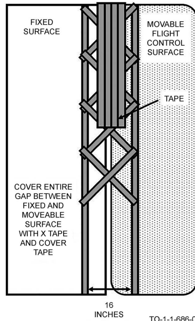
Figure 4-6. "X" Pattern for Control Surfaces
