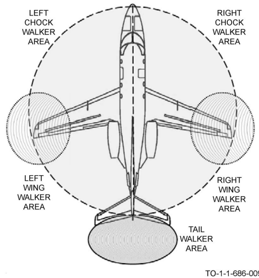
Figure 7-1. General Chock, Wing and Tail Walker Areas
