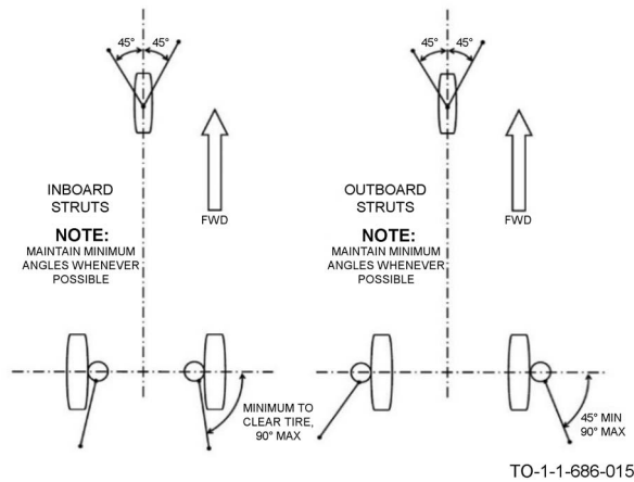
Figure 7-7. Cable Angular Relationship to Aircraft
