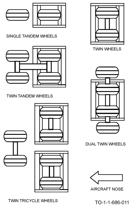
Figure 7-3. Chocking with Slats
