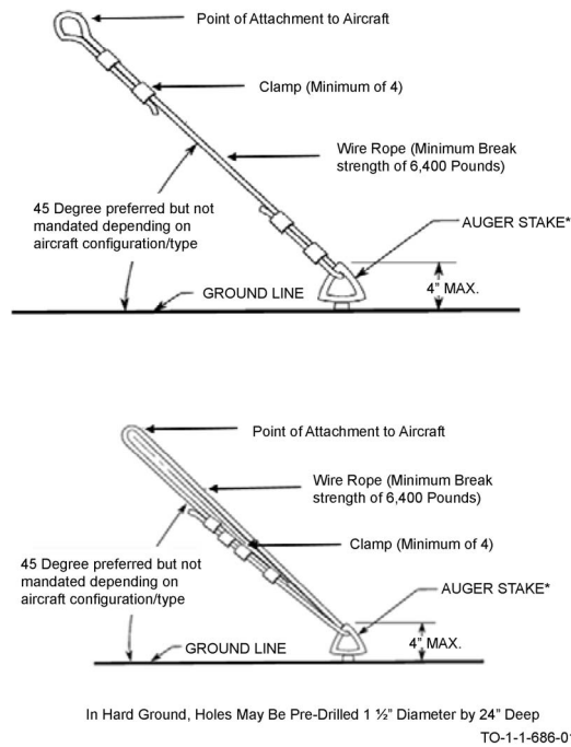
Figure 7-8. Cable Mooring Attachment
