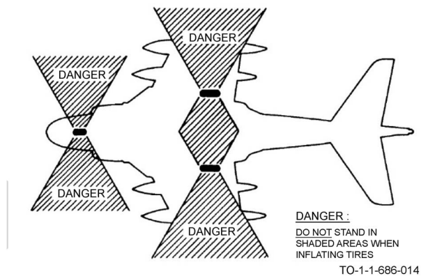
Figure 7-6. Tire Inflation Danger Areas
