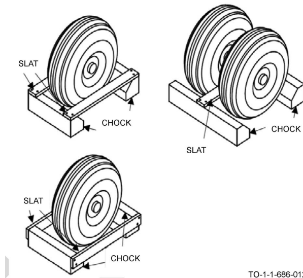
Figure 7-4. Chocks with Slats Attached
