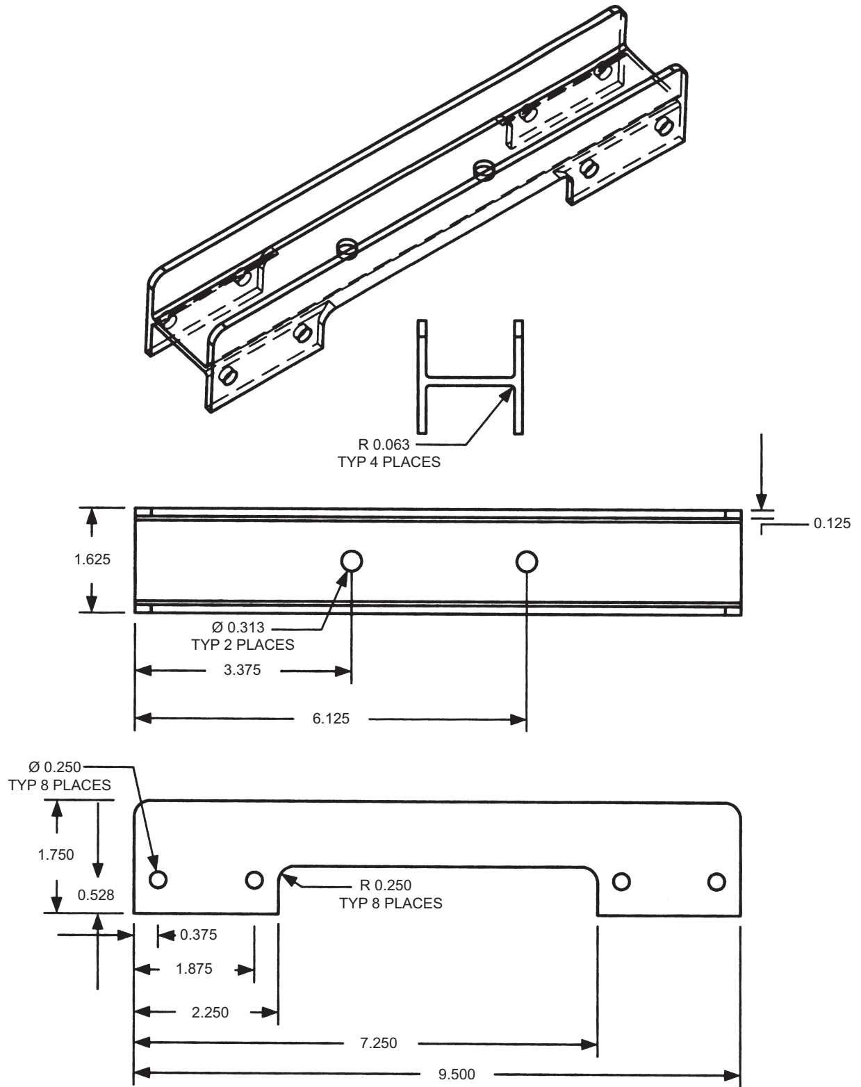
Figure 5-2. Exhaust Purge Adapter (Sheet 9)
