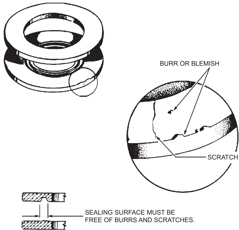
Figure 9-12. O-Ring Fitting Inspection
