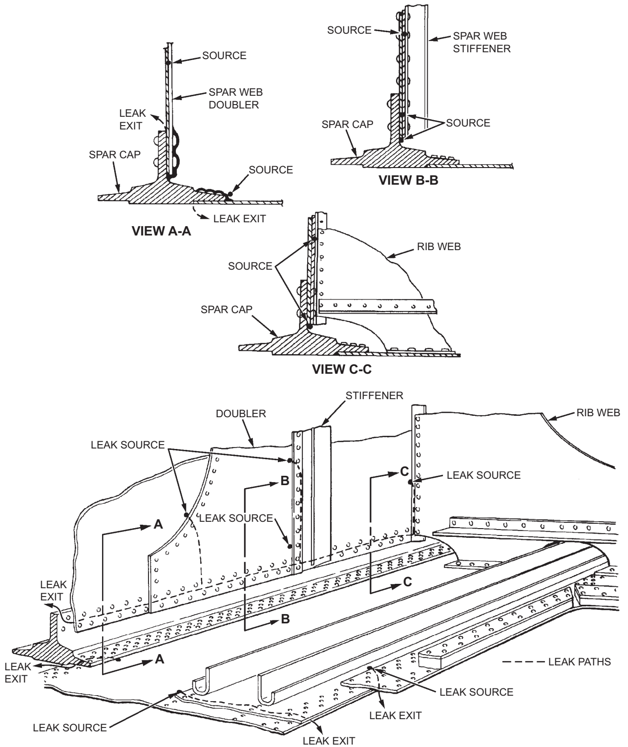
Figure 6-16. Examples of Long Leak Paths
