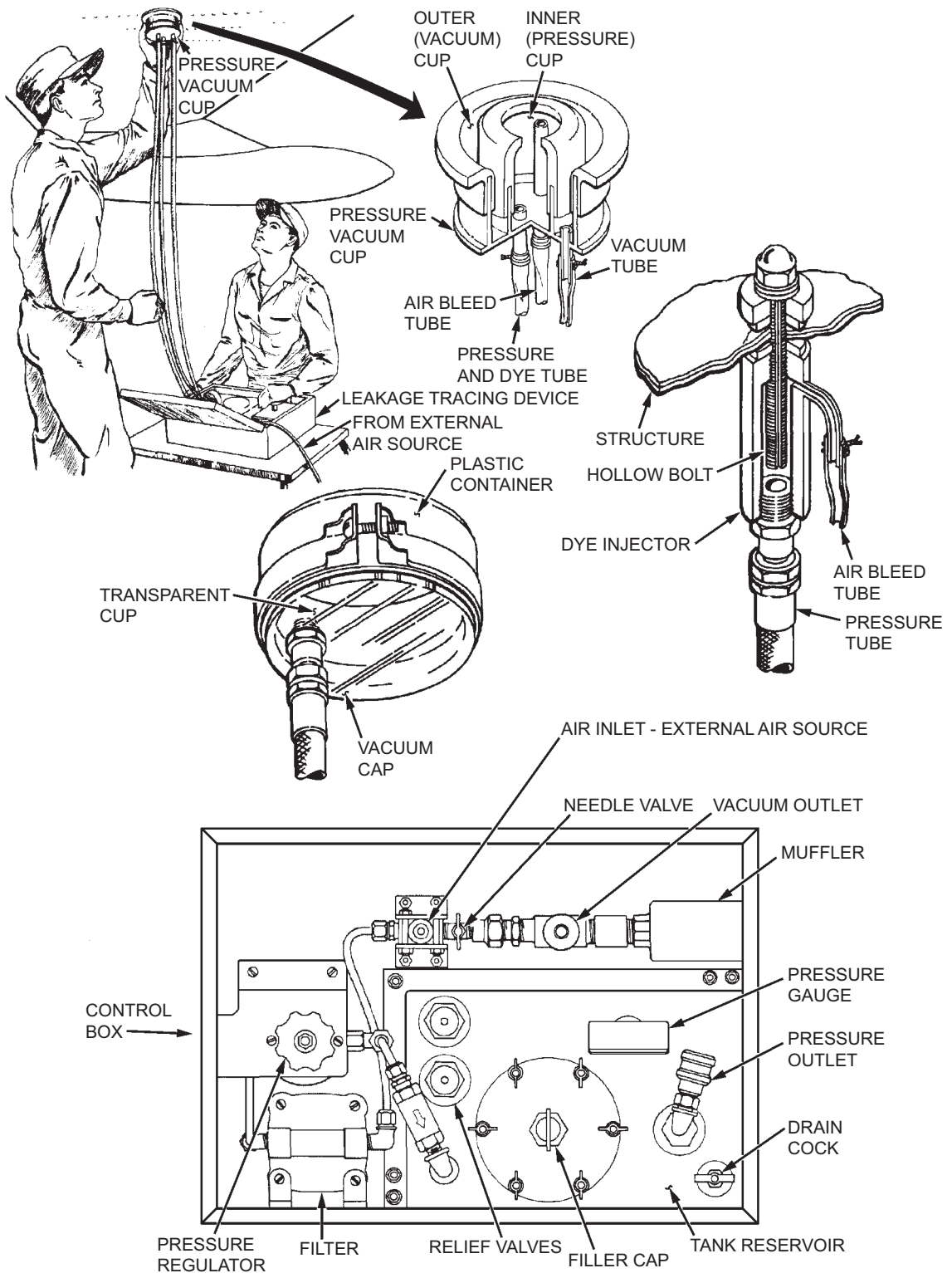
Figure 6-23. Dye Injection Method
