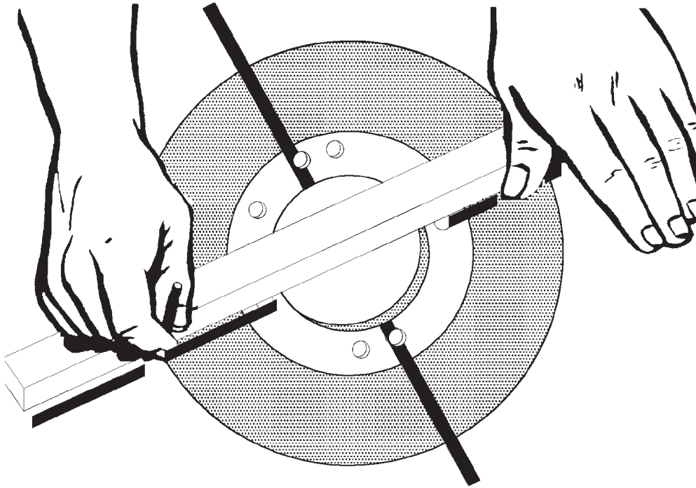
Figure 9-31. Locating Fitting
