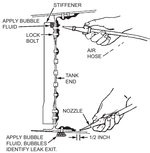
Figure 6-22. Blow Back Method
