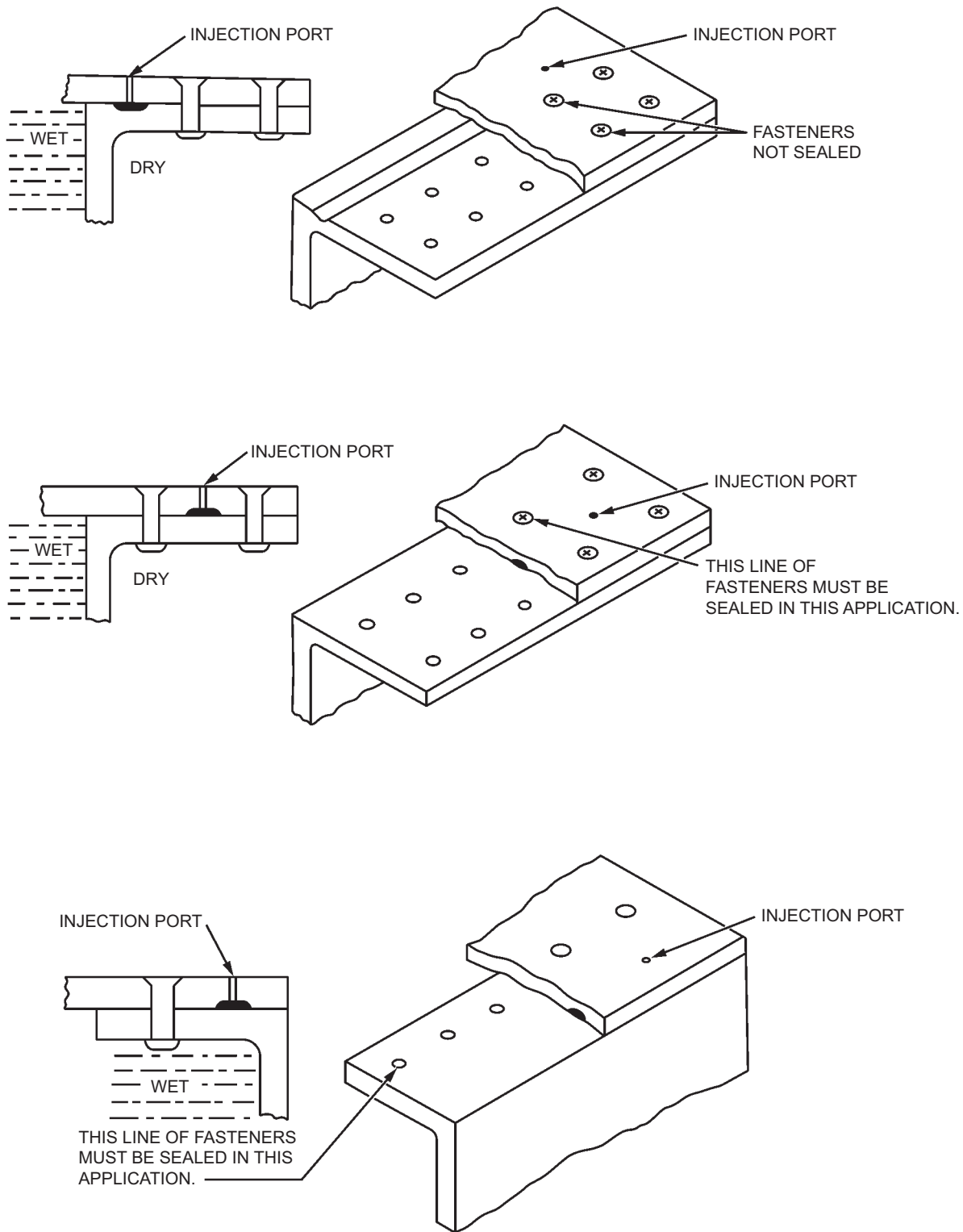
Figure 6-4. Typical Locations of Grooves/Channels (Sheet 1 of 2)
