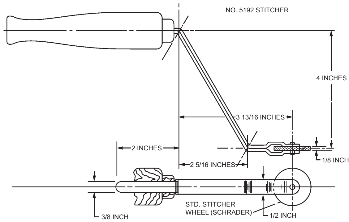
Figure 8-7. Horizontal Sticher
