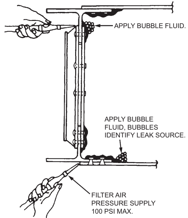
Figure 6-22. Blow Back Method
