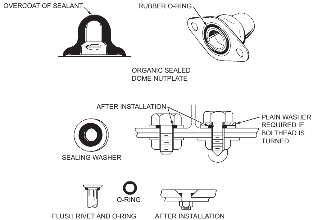
Figure 6-11. Typical Fastener Seal
