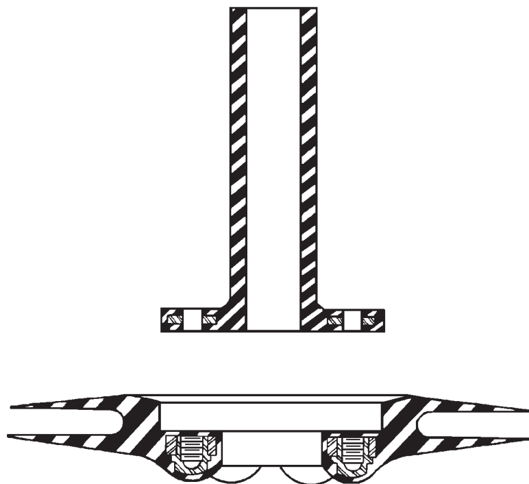
Figure 9-27. Two-Phase Fitting
