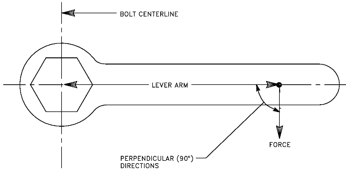
Figure 3-1. Simple Torque Problem
