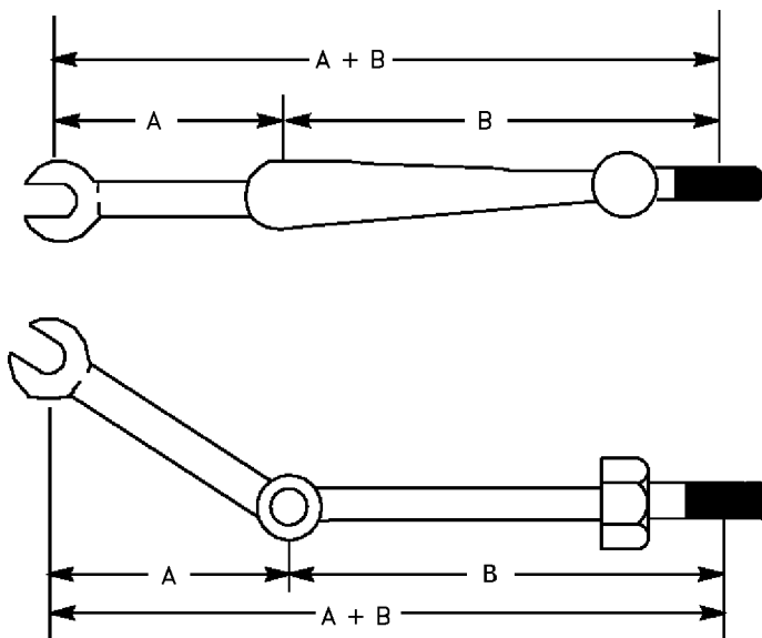
Figure 6-1. Extension Used When Total Length Exceeds Handle Length
