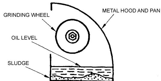
C TYPE OF DUST COLLECTOR FOR SMALL WHEELS USED ONLY INTERMITTENTLY AND WHEN SMALL AMOUNTS OF METAL ARE REMOVED.
